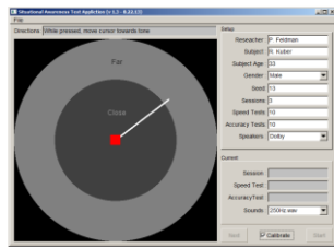
Figure 2: Application Interface
